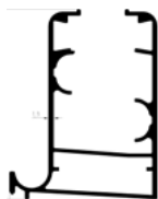
Dropper Super Case Profile
