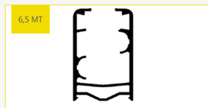
Case Profile
