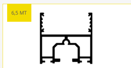
Wing Profile
